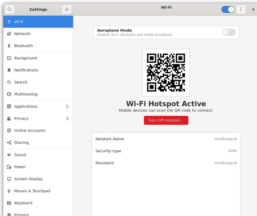
Figure 43 Hotspot active
