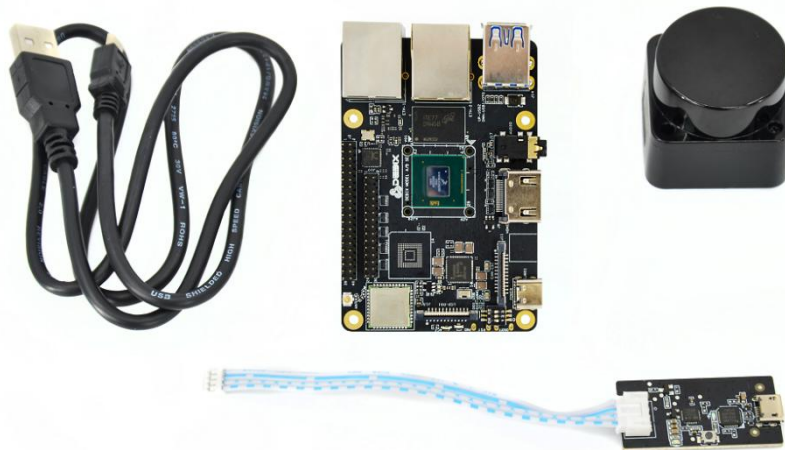
Figure 57
