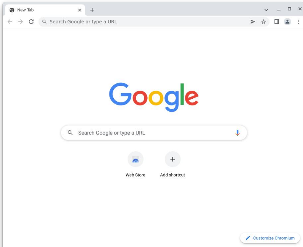
Figure 35 Chromium-browser
