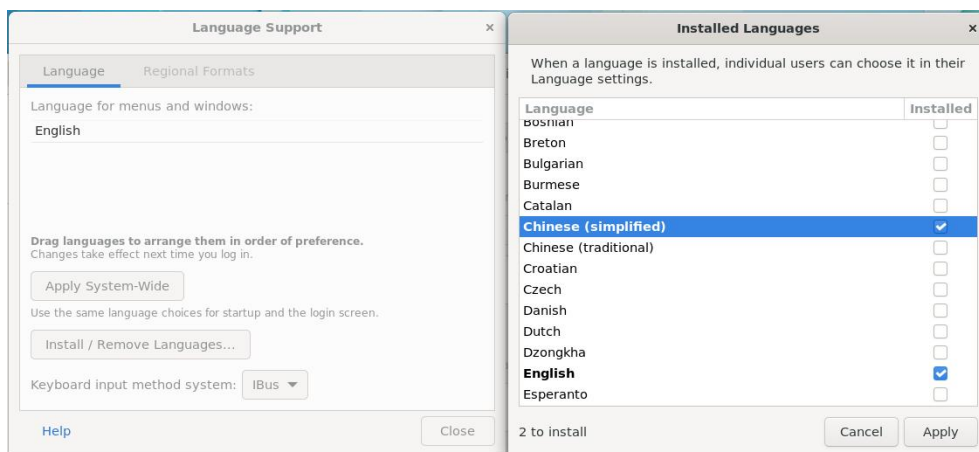
Figure 48 Languages option
