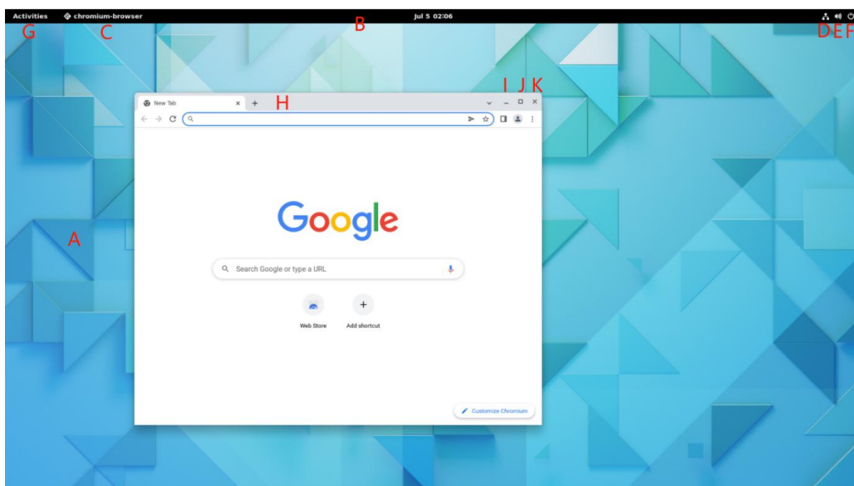
Figure 36 System Desktop
