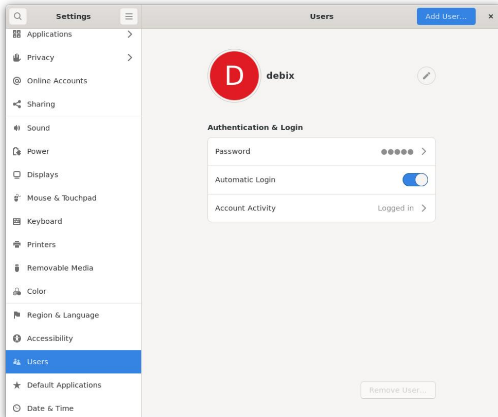
Figure 37
