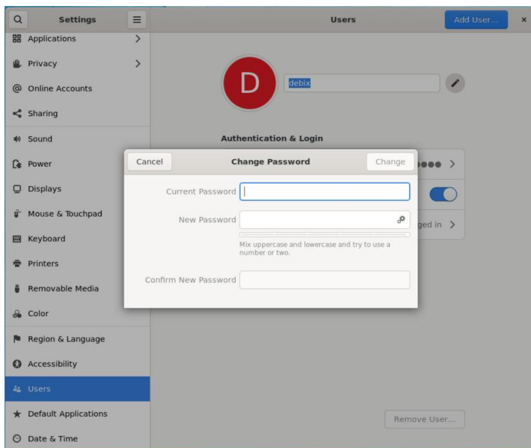
Figure 38 Change Password
