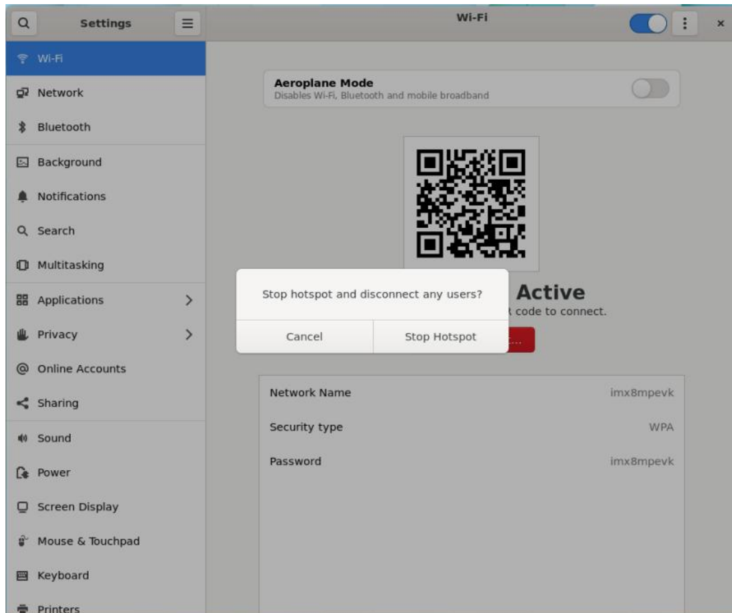
Figure 44
