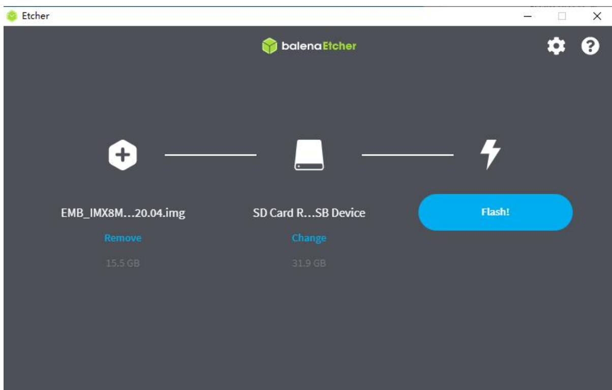
Figure 29
