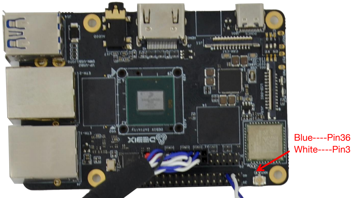
Figure 53 Connect LVDS screen cable to DEBIX Infinity
