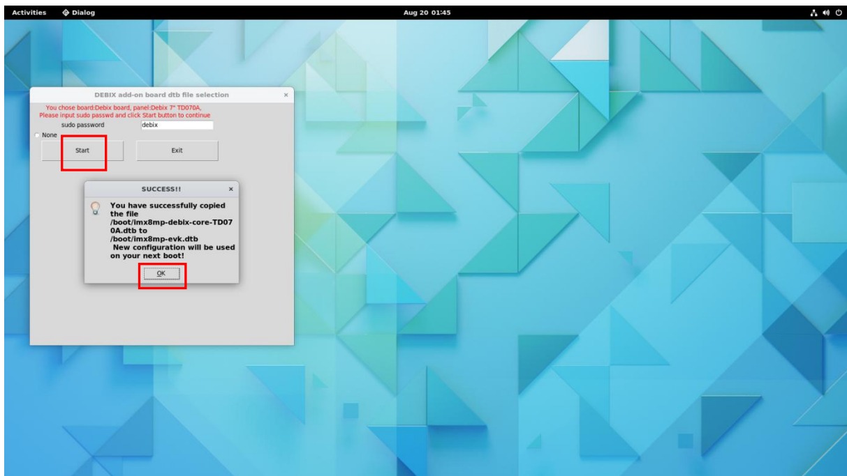
Figure 72
