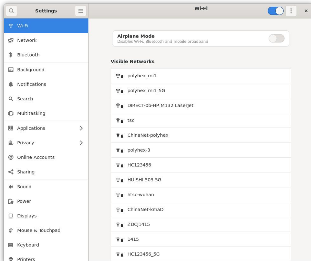
Figure 40 Wi-Fi interface
