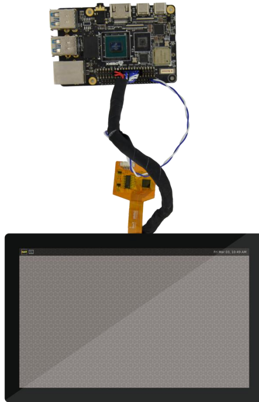
Figure 56
