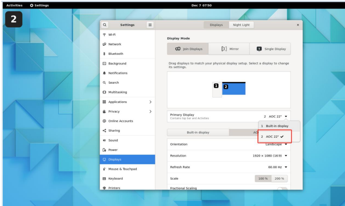
Figure 73
