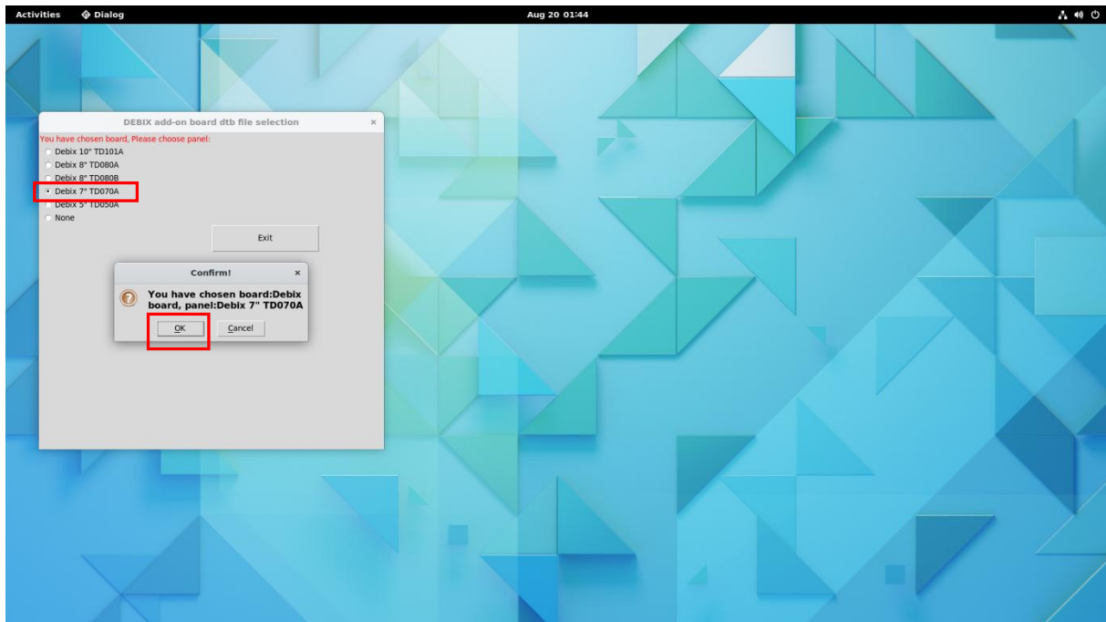
Figure 71
