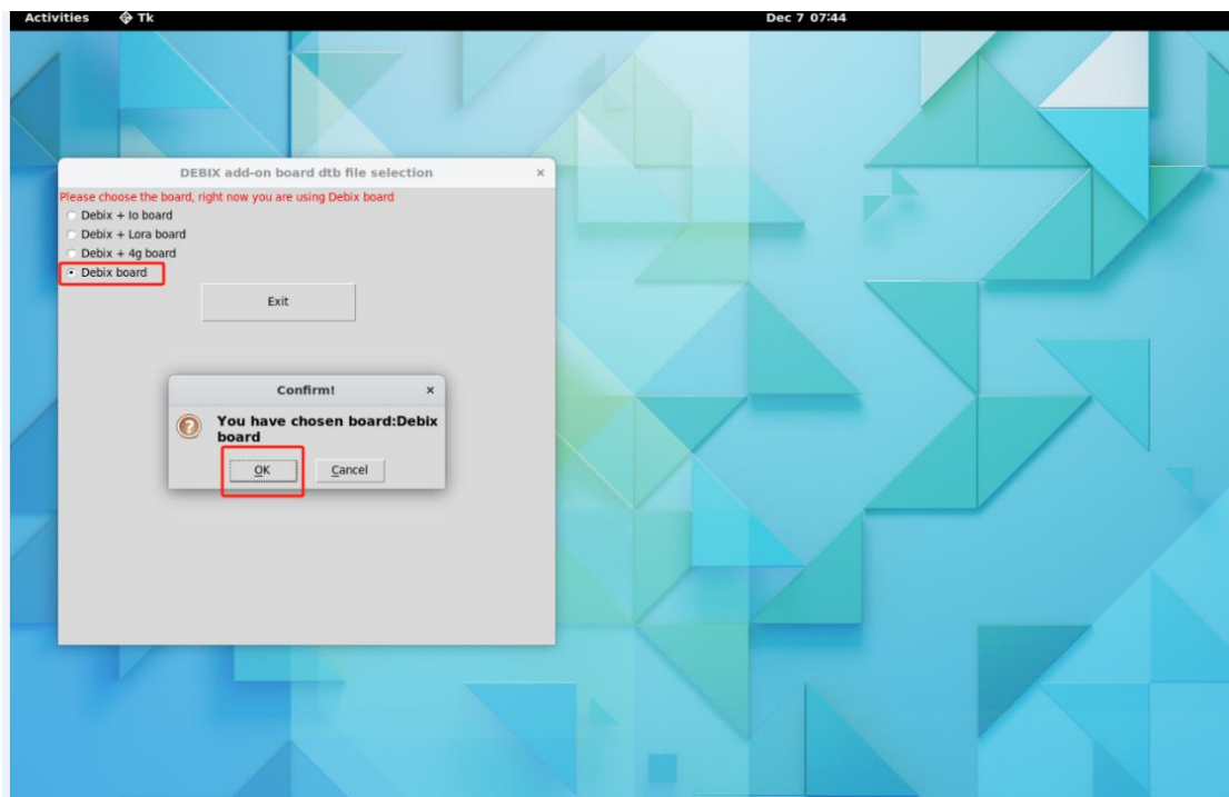
Figure 70
