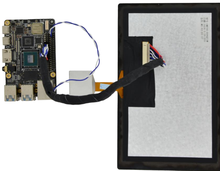
Figure 55 LVDS screen to DEBIX Infinity completed
